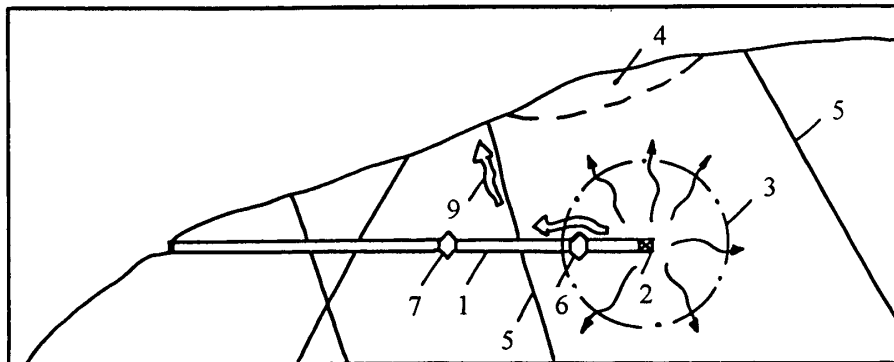
Figure 20. Illustration of gas release through a tectonic fault that intersects the tunnel between the first and second stemming sections: 1- tunnel works; 2- zero room; 3- damage zone radius; 4- spill zone; 5- tectonic faults; 6 and 7- first and second stemming; 9- gas flow through the tectonic fault.
